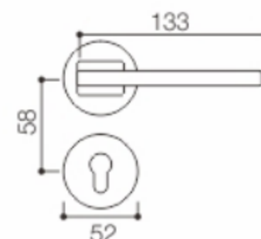
Size diagram
