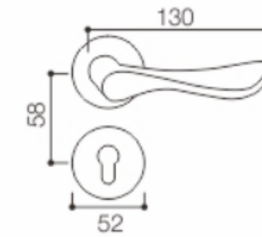
Size diagram
