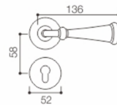
Size diagram
