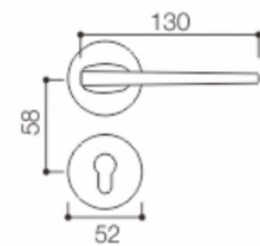
Size diagram
