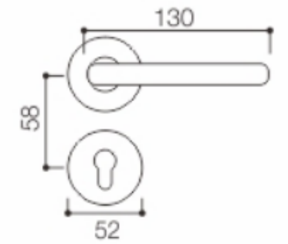
Size diagram
