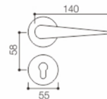
Size diagram
