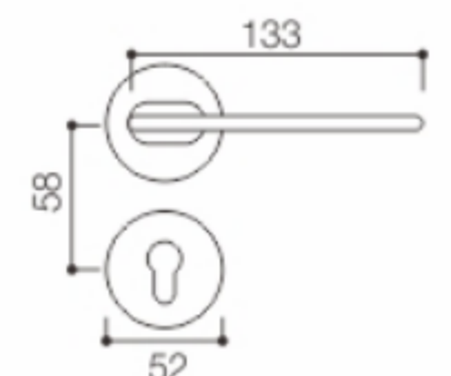
Size diagram
