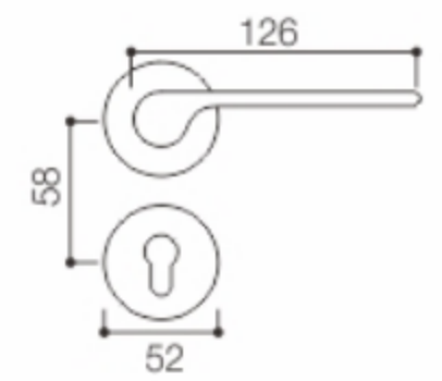
Size diagram
