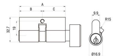
Euro Profile Thumb Turn Cylinder
