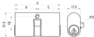
UK Oval Double Cylinder
