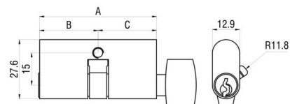
Italian Thumb Turn Cylinder
