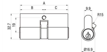
Euro Profile Double Cylinder
