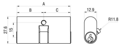
Italian Oval Double Cylinder
