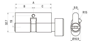
Euro Profile Thumb Turn Cylinder
