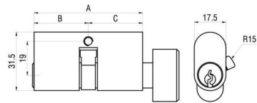
UK Oval Thumb Turn Cylinder
