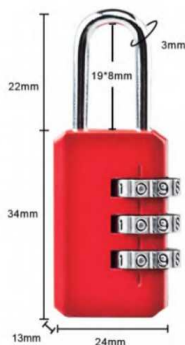
Item:8012 Size: 2.20*0.94*0.51in Material: Zinc alloy Weight: 22.8g
