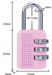
Item:8021 Size: 2.16*1.06*0.55in Material: Zinc alloy Weight: 35.8g
