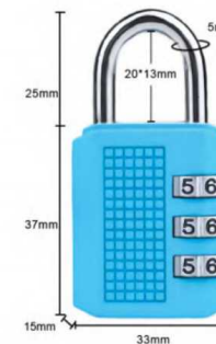
Item:8022 Size: 2.44*1.30*0.59in Material: Zinc alloy Weight: 52.4g
