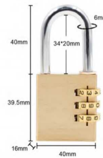
Item:8044 Size: 3.13*1.57*0.63in Material: Brass Weight: 143.3g
