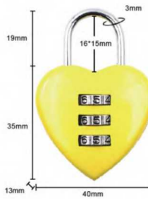
Item:8026 Size: 2.13*1.57*0.51in Material: Zinc alloy Weight: 25.6g
