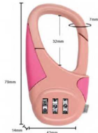
Item:8054 Size: 3.11*1.65*0.55in Material: Zinc alloy Weight: 64.1g
