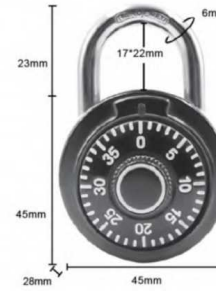
Item:8056B Size: 2.68*1.77*1.10in Material: Zinc alloy Weight: 85g
