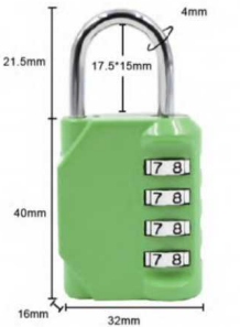
Item:8023B Size: 2.42*1.26*0.63in Material: Zinc alloy Weight: 50.4g
