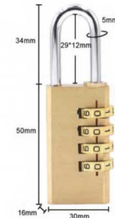
Item:8043 Size: 3.31*1.18*0.63in Material: Brass Weight: 106g
