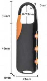
Item:8064 Size: 2.56*0.82*0.35in Material: Zinc alloy Weight: 26g
