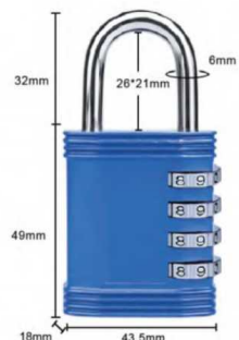
Item:8017A Size: 3.19*1.71*0.71in Material: Zinc alloy Weight: 129.4g
