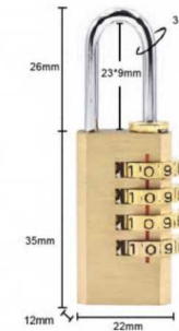
Item:8041 Size: 2.40*0.87*0.53in Material: Brass Weight: 56.5g
