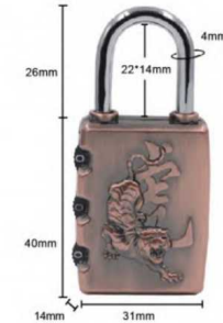
Item:8028 Size: 2.60*1.22*0.55in Material: Zinc alloy Weight: 38g
