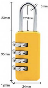
Item:8066 Size: 2.40*0.94*0.47in Material: Zinc alloy Weight: 24g
