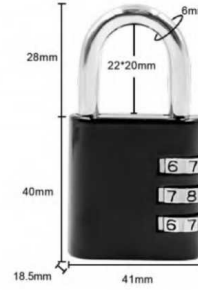
Item:8082 Size: 2.68*1.61*0.73in Material: Zinc alloy Weight: 87.2g
