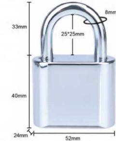
Item:8083 Size: 2.87*2.05*0.94in Material: Zinc alloy Weight: 232g
