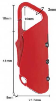
Item:8015 Size: 2.44*0.92*0.31in Material: Zinc alloy Weight: 19.6g
