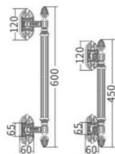
Lever Handle HK1623 HK2623-1
