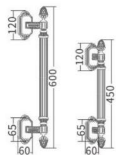
Lever Handle HK1624 HK2624-1
